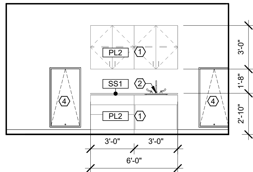
5 RESEARCH SUPPORT - NORTH A708 1/4" = 1'-0"
