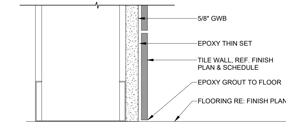
8 A503 6" = 1'-0" INTERIOR DETAIL - TILE WALL BASE
