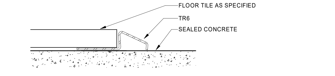
6 A503 12" = 1'-0" INTERIOR DETAIL - TR6 FLOOR TILE TO CONCRETE
