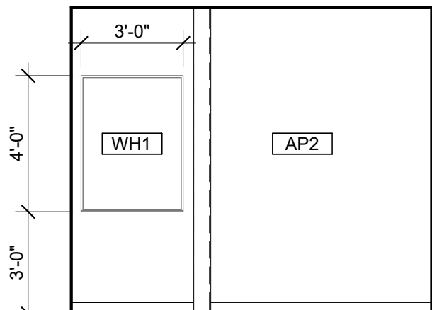
13 TYP. 4P HUDDLE SPACE - EAST 1/4" = 1'-0" TYPICAL AT 112, 228, 230
