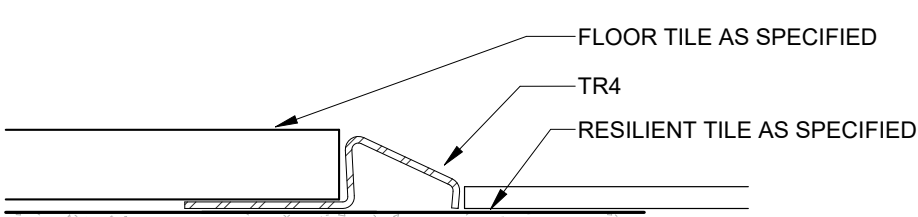
4 A503 12" = 1'-0" INTERIOR DETAIL - TR4 RESILIENT TO FLOOR TILE
