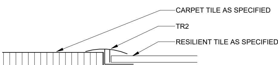
2 A503 12" = 1'-0" INTERIOR DETAIL - TR2 CARPET TO RESILIENT
