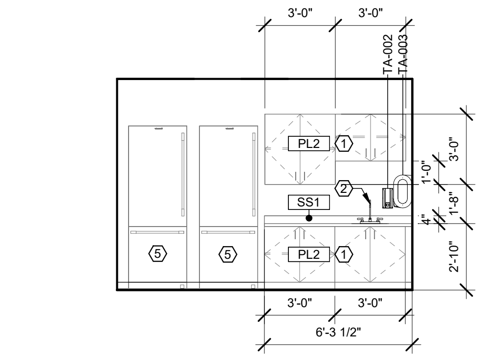
2 FACULTY GATHERING - WEST A708 1/4" = 1'-0"
