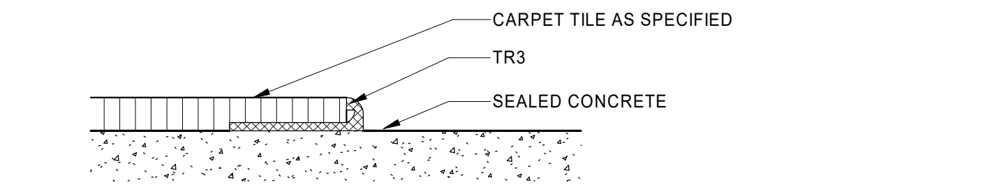
3 A503 12" = 1'-0" INTERIOR DETAIL - TR3 CARPET TO CONCRETE
