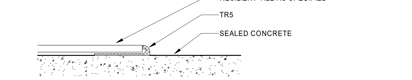
5 A503 12" = 1'-0" INTERIOR DETAIL - TR5 RESILIENT TO CONCRETE
