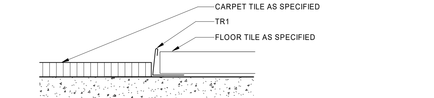
1 A503 12" = 1'-0" INTERIOR DETAIL - TR1 CARPET TO FLOOR TILE
