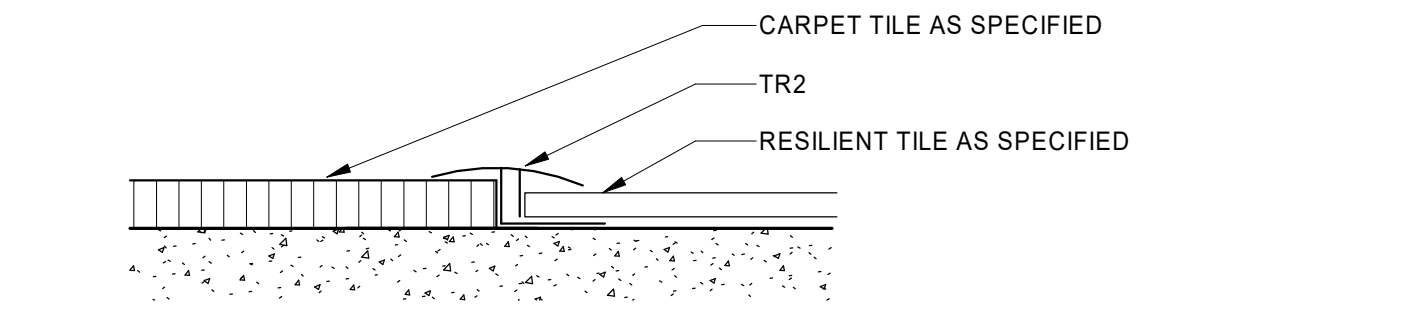
2 A503 12" = 1'-0" INTERIOR DETAIL - TR2 CARPET TO RESILIENT
