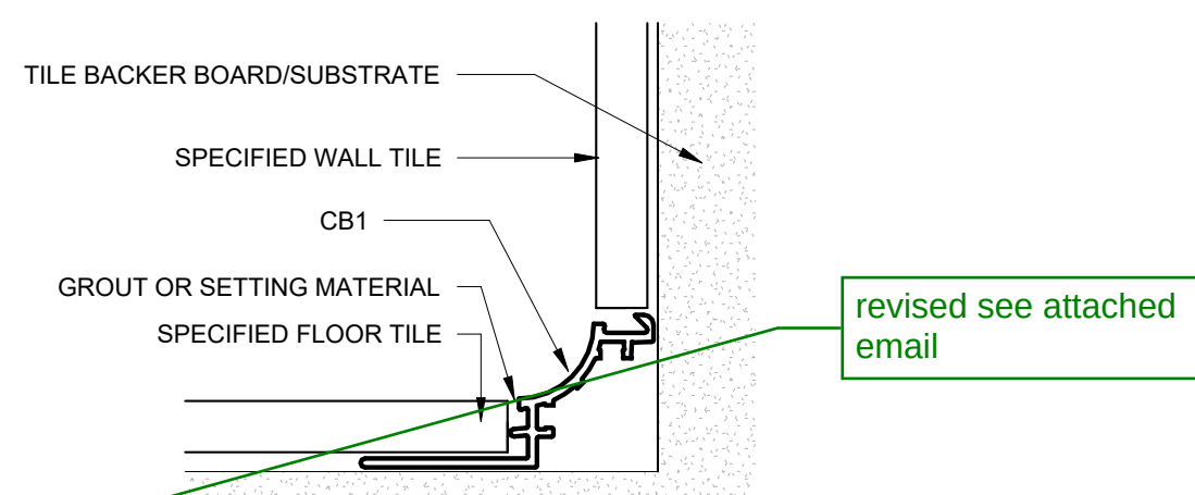
7 A503 12" = 1'-0" INTERIOR DETAIL - TILE COVE BASE
