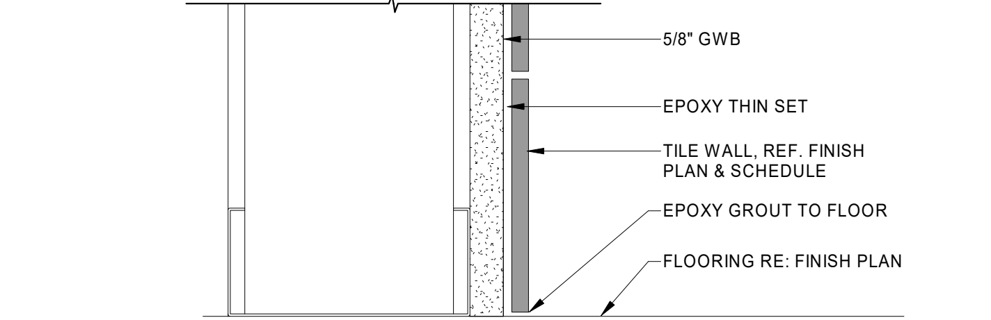
8 A503 6" = 1'-0" INTERIOR DETAIL - TILE WALL BASE
