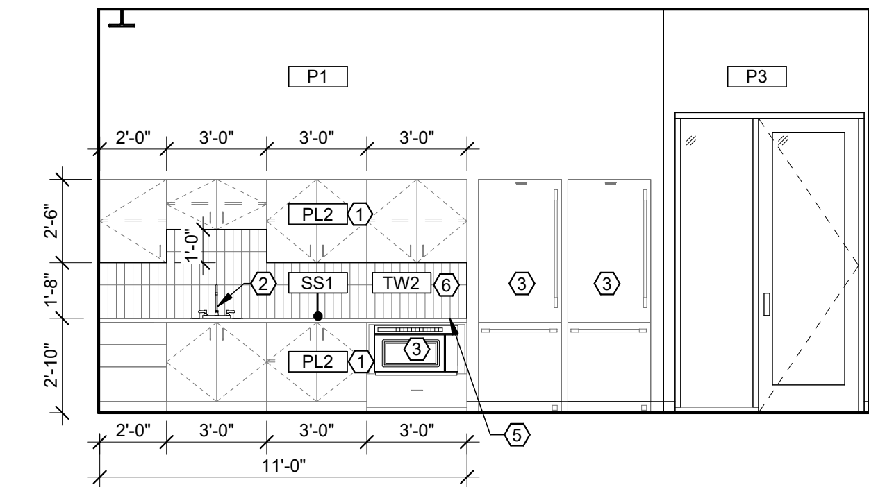
1 NOURISHMENT 104 - NORTH A706 1/4" = 1'-0"
