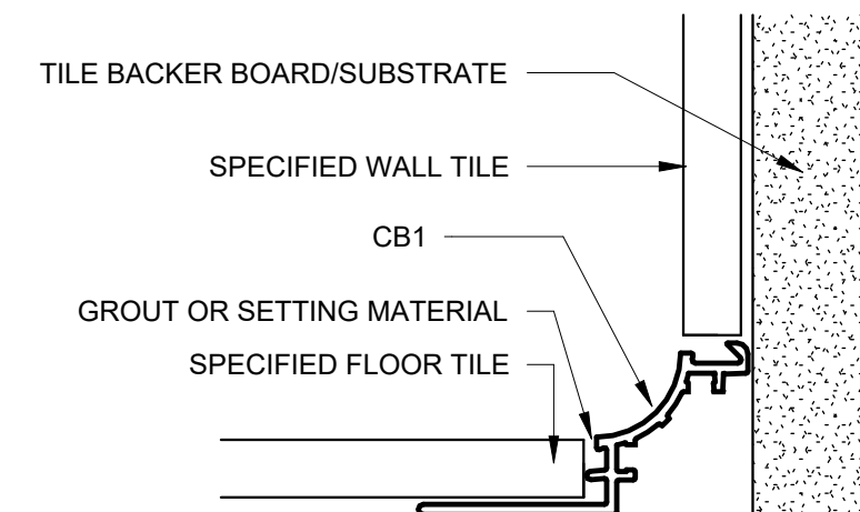
7 A503 12" = 1'-0" INTERIOR DETAIL - TILE COVE BASE
