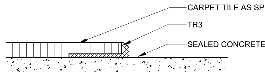
3 A503 12" = 1'-0" INTERIOR DETAIL - TR3 CARPET TO CONCRETE
