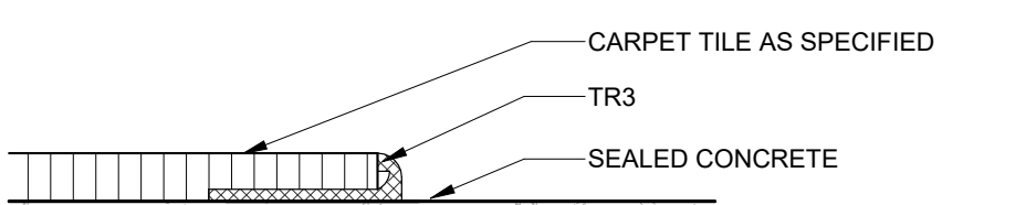
3 A503 12" = 1'-0" INTERIOR DETAIL - TR3 CARPET TO CONCRETE
