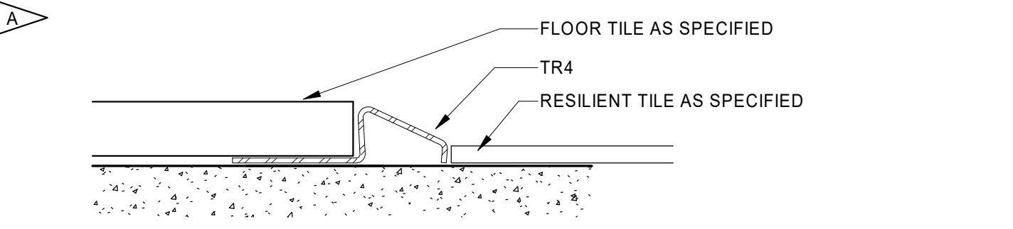
4 A503 12" = 1'-0" INTERIOR DETAIL - TR4 RESILIENT TO FLOOR TILE
