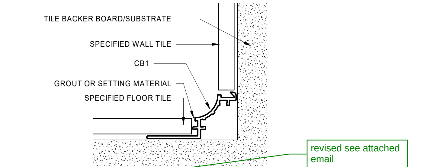
7 A503 12" = 1'-0" INTERIOR DETAIL - TILE COVE BASE
