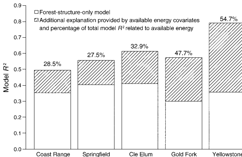
FIG. 5. Model R 2 and percentage of the total model R 2 resulting from the addition of five predictors of available energy to a five-predictor forest structure model at each landscape.
